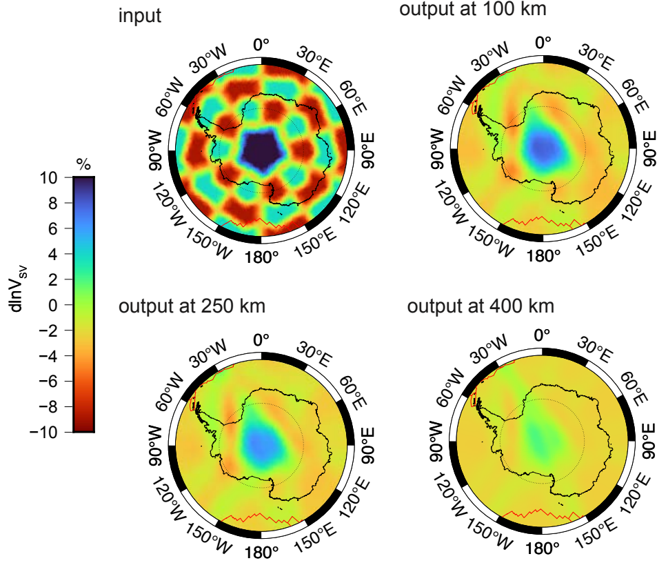
Figure S4: Synthetic tests with isotropic checkerboard input model and the corresponding isotropic output models at 100 km, 250 km depth, and 400 km. The input cells span 30 degrees in longitude and 8 degrees in latitude. The anomaly at the pole has a radius of 8 degree.
