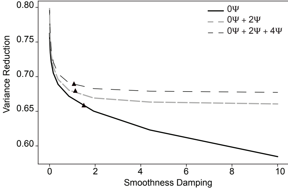
Figure S3: Example of damping parameter selection based on the L-curve method. The optimal damping parameters are selected at the elbow of the curves and are denoted by triangles. We first searched for the damping parameters for the 0\Psi -term. The 0\Psi + 2\Psi curve was obtained by fixing the selected isotropic damping parameter and changing the 2\Psi -term damping. The 0\Psi + 2\Psi + 4\Psi curve resulted from varying the 4\Psi damping parameter while fixing the isotropic and 2\Psi -term damping parameters.
