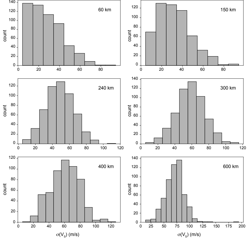
Figure S2: Distribution of path-averaged velocity V_{SV}(z) standard deviations at different depths. All paths shown in Fig. 2 of the main text were included, and the standard deviation for each path is calculated from the ensemble of models obtained by our MCMC algorithm.
