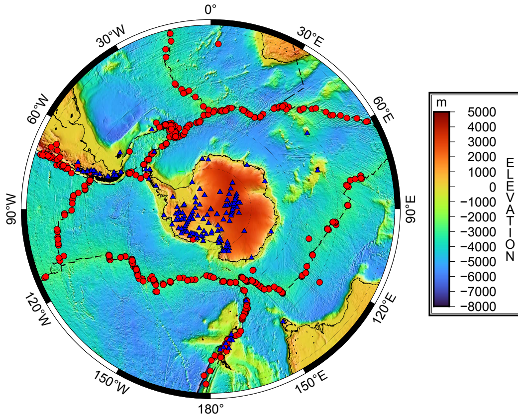
Figure S1: Maps of the selected event location (red circles) and stations (blue triangles) superimposed on bathymetry and topography Tozer et al. (2019). Ocean ridges are shown by the dashed black lines.
