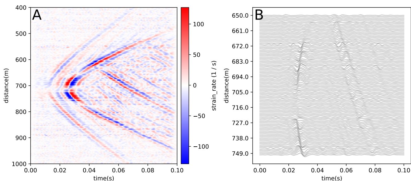
Figure 2 Waterfall (left) and wiggle (right) plots produced by Listing 2.
