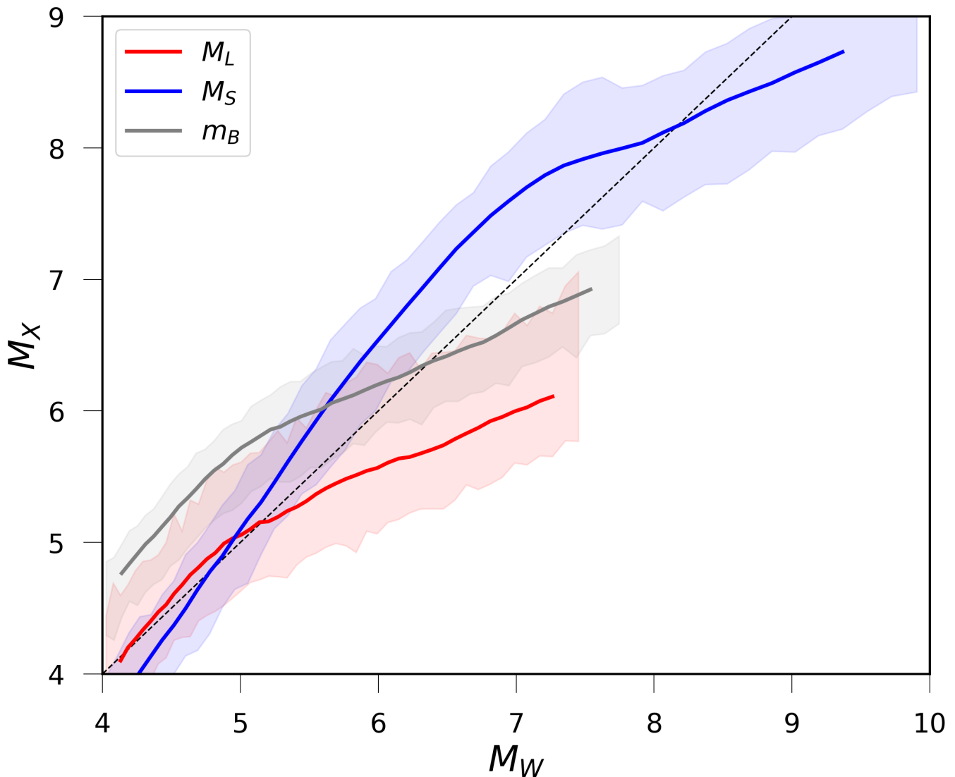
Figure S.2 Predicted relations between various magnitude scales in the range from M_W 4 to 9.5. 15% percentiles are plotted by transparent regions.
