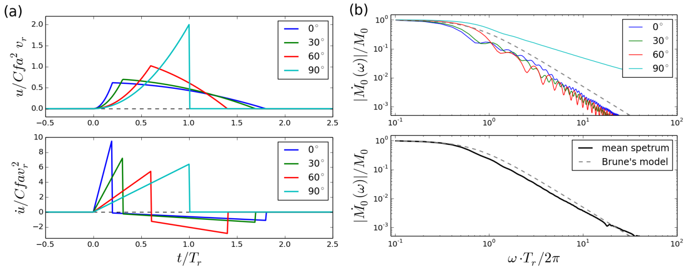
Figure S.1 (a) Displacement (up) and velocity pulses (down, both normalized for geometrical spreading and radiation) of the circular rupture model for different angles \vartheta . (b) The normalized amplitude spectra of the associated apparent moment rate functions. The upper panel shows spectra for specific values of \vartheta , while the lower shows the mean spectrum (black) in comparison with the Brune's spectrum (dashed, gray) assuming an effective rise time of 1.5 \cdot T_r , where T_r is the rupture time. Figures are from Dahm (2022): Earthquake sources and rupture processes in seismology and volcanology . Lecture Notes, University of Potsdam.
