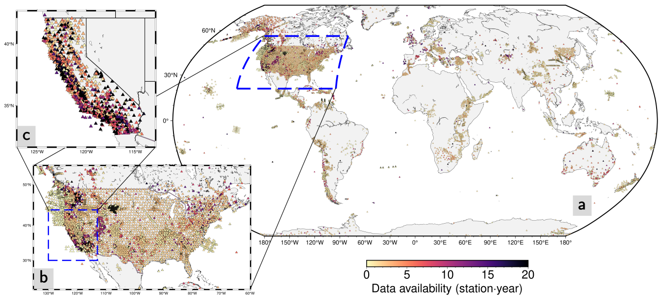
Figure 1 Map of stations, displayed as triangles and color coded according to the Data availability in station-years included in EarthScope, NCEDC, and SCEDC archives. Panel (a) shows the distribution of global station data availability. Panel (b) shows a detailed view of stations in the United States, while Panel (c) shows data availability in California.
