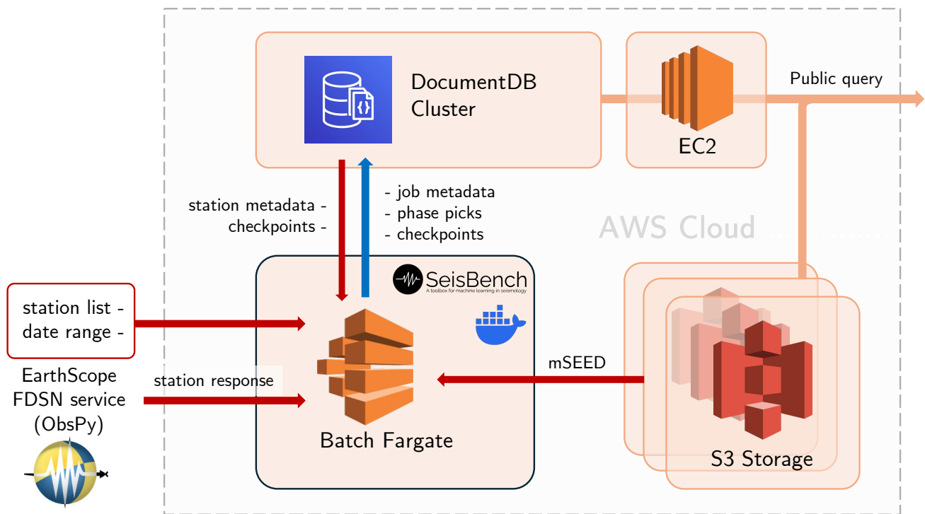
Figure 2 The scalable cloud-native workflow for seismic phase picking. Containerized jobs are submitted to AWS Batch, which loads miniSEED seismic waveforms directly from AWS S3 buckets. Phase arrivals were identified with PhaseNet through the SeisBench implementation. A DocumentDB cluster is employed to store job metadata, picks, and checkpoints. Finally, an EC2 instance is used to provide a public database query service.
