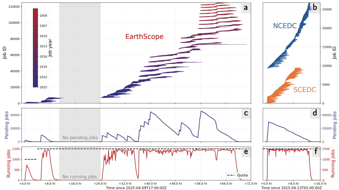
Figure 3 Detailed job run history for the EarthScope, NCEDC, and SCEDC dataset. Panel (a) shows the Job ID as a function of time, color-coded by year the data was recorded, for the EarthScope dataset. Panel (b) shows the job progression for the NCEDC and SCEDC datasets. Panels (c) and (d) show the pending jobs as a function of time. Panels (e) and (f) show the running jobs as a function of time. The horizontal dashed line represents the job quota.
