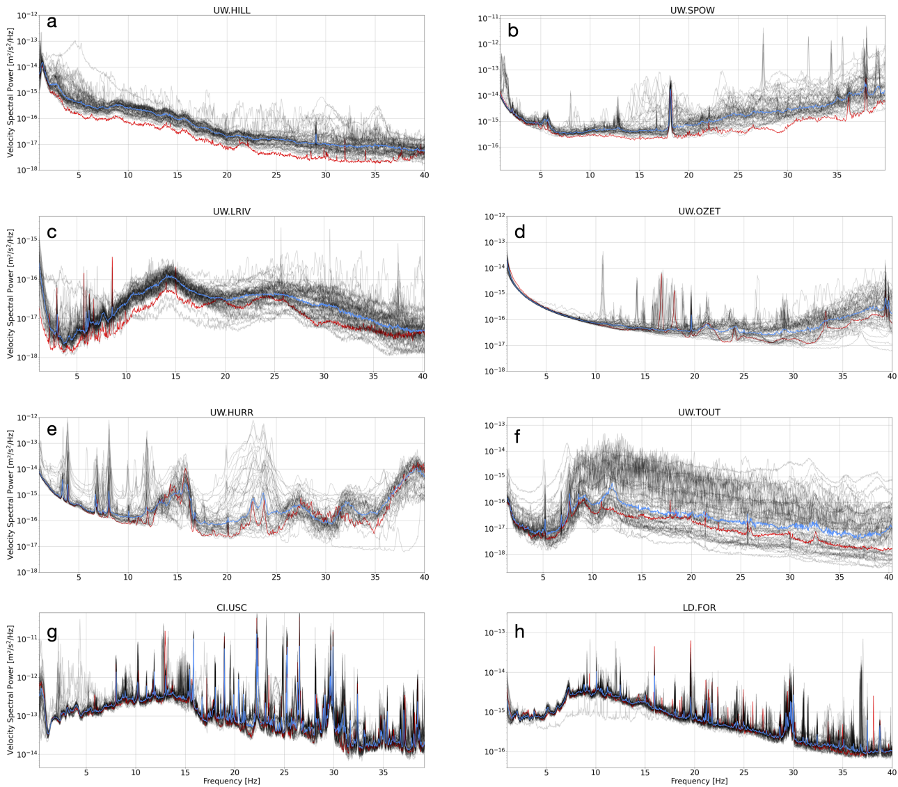
Figure 2 PPSDs for eight stations farther afield from Seattle: a) HILL in the semi-rural area of La Conner, b) SPOW on the edge of metropolitan Spokane in eastern Washington, c) LRIV a few kilometres outside Port Angeles, d) OZET in the small hamlet of Ozette on the Olympic Peninsula, e) HURR on the uninhabited Hurricane Ridge in the Olympic National Park, f) TOUT on the uninhabited slopes of Mount St Helens; and for external comparison two stations other non-Washington major cities: CI.USC at the University of Southern California in Los Angeles in g) and LD.FOR in Fordham, New York City in h) . As per Fig. 1, in each panel, each black line is the PPSD for a non-Superbowl Sunday. The blue line is the median of all Sundays, including the Superbowl Sunday. The red line is the Superbowl Sunday (February 8, 2026).
