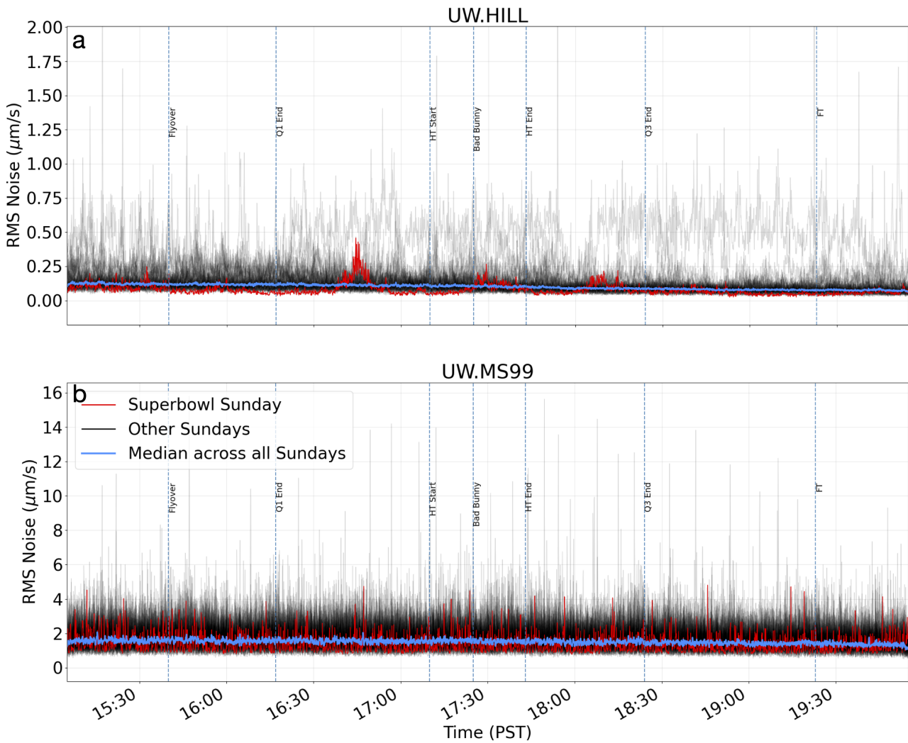
Figure 3 Time-resolved noise levels at stations a) HILL and b) MS99. Major events including the flyover/kickoff, end of each quarter, half-time, and full-time are shown; along with the timing of Bad Bunny’s show. No particular trends are apparent. The bandwidth here is 1-20 Hz and the window length is 5 s.
